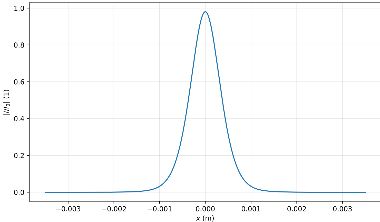
Intensity profile I(x, y = 0, z = 2.468m)/I_0 , \text{Pin}=0.7\text{Pcr} , artificial time
